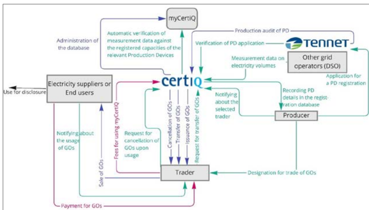
Figure 47: Main processes in the GO system with interactions between actors in the Netherlands (own representation)
